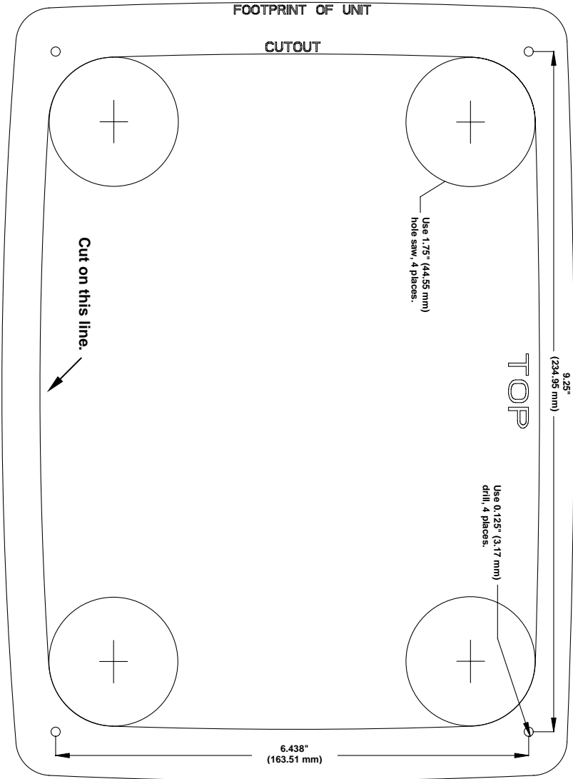
FM-11 dash mounting template, part number 988-0154-691. NOTE: This drawing is not to scale and is for illustration only. Always verify template print dimensions before use.
